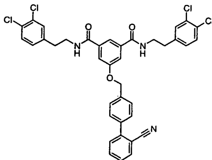
Compound # 21
